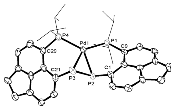
Figure 3. Molecular structure of 4 . Thermal ellipsoids are set at 40% probability; hydrogen atoms are omitted for clarity. The iPr groups on P1 and P4 (two on each) are drawn as wireframe for clarity.
